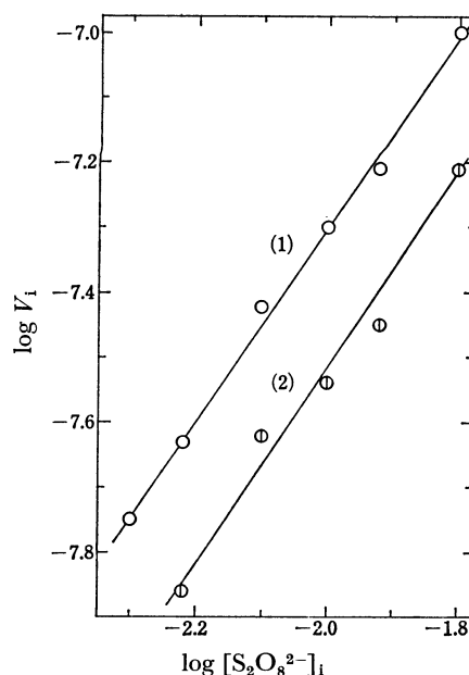
Fig. 2. Plot of \log V_i vs. \log [\text{S}_2\text{O}_8^{2-}]_i .
